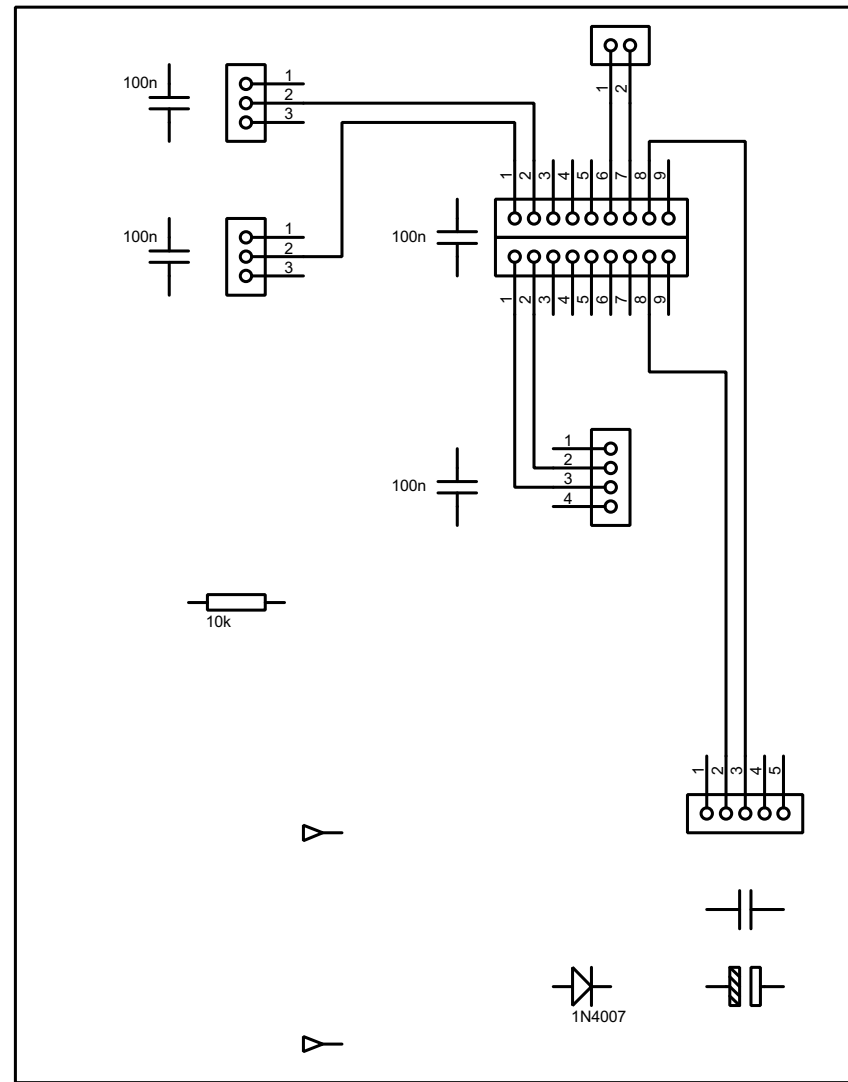
FRONT BOARD
