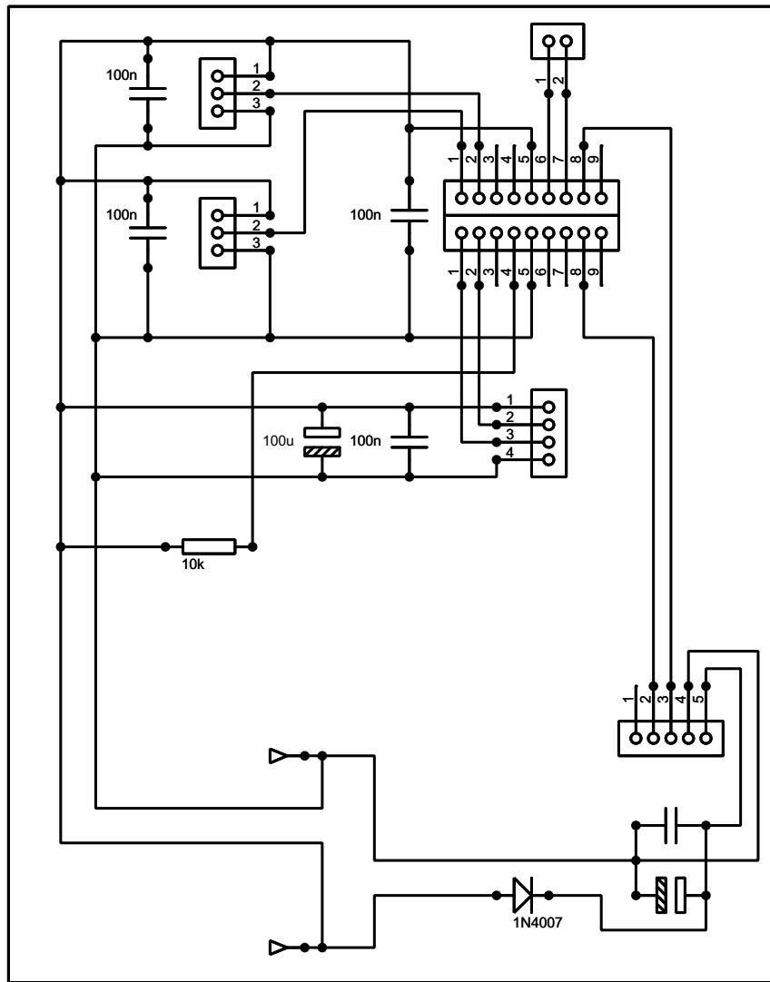
Full Circuit
