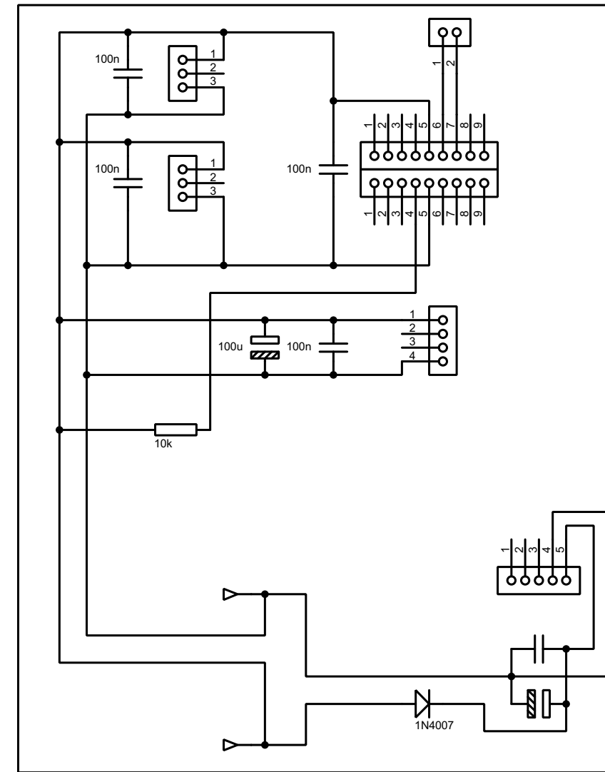
BACK BOARD
